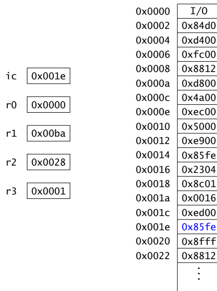
Figure 1: A block diagram of the CS52 Machine. The registers are on the left, and a portion of memory is on the right. Register ic has the value 0x001e , and the word at that address—shown in blue—is the instruction that is about to be executed. All values are given in hexadecimal.
