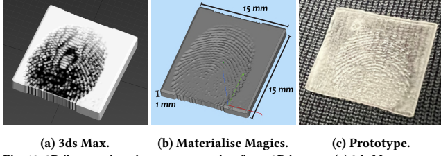
Fig. 12: 3D fingerprint pieces construction from 2D images. (a) 3ds Max converts the 2D grayscale fingerprint images to 3D models, (b) Materialise Magics to reshape the 3D models to 15\text{mm} \times 15\text{mm} \times 1\text{mm} , and (c) A prototype of 3D print fingerprint pieces from 3D printer.
