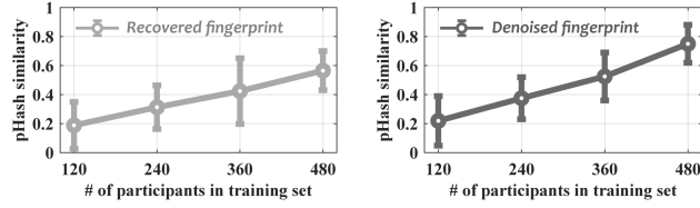
Fig. 22: pHash similarity of recovered and denoised fingerprints with different numbers of participants in the training set (§ 7.3).
