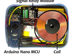
Fig. 7: Compromised power bank.
