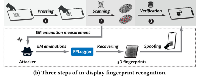
Fig. 3: A motivating example: a user places the finger on the in-display fingerprint sensor to unlock the smartphone. The attacker can leverage the EM emanations to recover the user's fingerprint to build 3D pieces to spoof the in-display fingerprint sensor.
