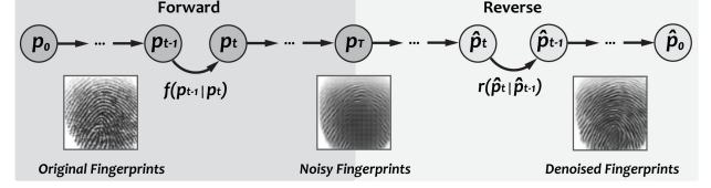
Fig. 11: Illustration of the denoising diffusion model. Note that the noisy fingerprint images are the output of the convolutional VAE model (§ 4.5) and are being denoised in the reverse process.
