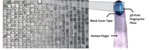
Fig. 13: Illustration of the experimental setup leveraging 3D printed fingerprint pieces to register the user and unlock the smartphone.
