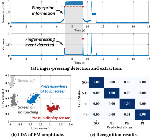
Fig. 8: Finger-pressing event detection and extraction (a), and false finger-pressing rejection based on the LDA of EM amplitude (b) and the recognition results (c) (SO: Screen off, NT: Screen on, no touching, PE: Press elsewhere on the touchscreen, PI: Press the in-display fingerprint sensor).
