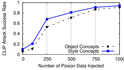
Figure 22. Attack success rate of the simple poisoning attack against LD-CC, measured by the CLIP classifier. The simple poisoning attack is more effective at corrupting style concepts than object concepts. The same applies to attacks against SD-V2, SD-XL, DeepFloyd.
